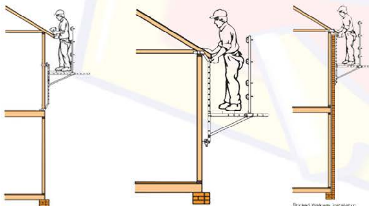
Bricked Walkway Installation
